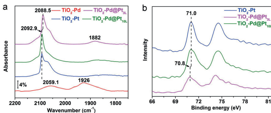
Figure 3. a) CO chemisorption DRIFTS spectra and b) XPS Pt 4f high-resolution spectra of TiO 2 -Pd@Pt 3L and TiO 2 -Pd@Pt 10L and TiO 2 -Pt and/or TiO 2 -Pd hybrid structures for comparison.
