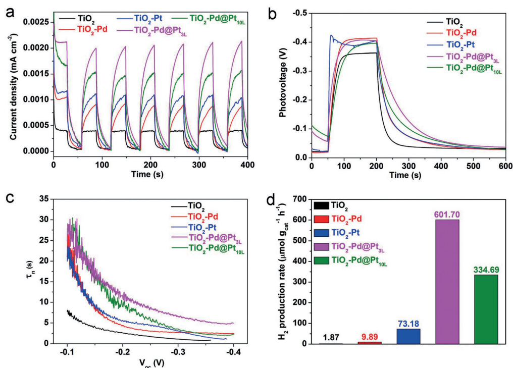
Figure 2. a) I-t curves of TiO 2 -Pd@Pt 3L and TiO 2 -Pd@Pt 10L in comparison with those of bare TiO 2 nanosheets, TiO 2 -Pd, and TiO 2 -Pt hybrid structures under UV light irradiation ( \lambda < 400 nm, 2.7 mWcm -2 ) at a bias potential of 0 V vs. Ag/AgCl. b) Transient OCVD measurements after exposure to UV light. c) Average lifetimes of the photogenerated carriers ( \tau_n ) obtained from the OCVD measurements. d) Photocatalytic H 2 evolution from water with the samples as catalysts under the same irradiation conditions.
